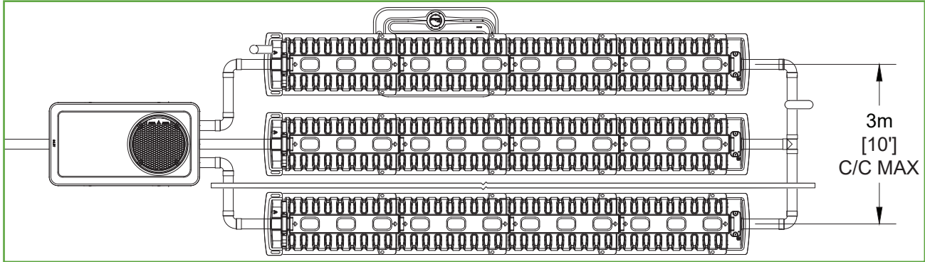
Figure 2: Configuration recommended for system width \leq 3m (10') – Remote vent example
