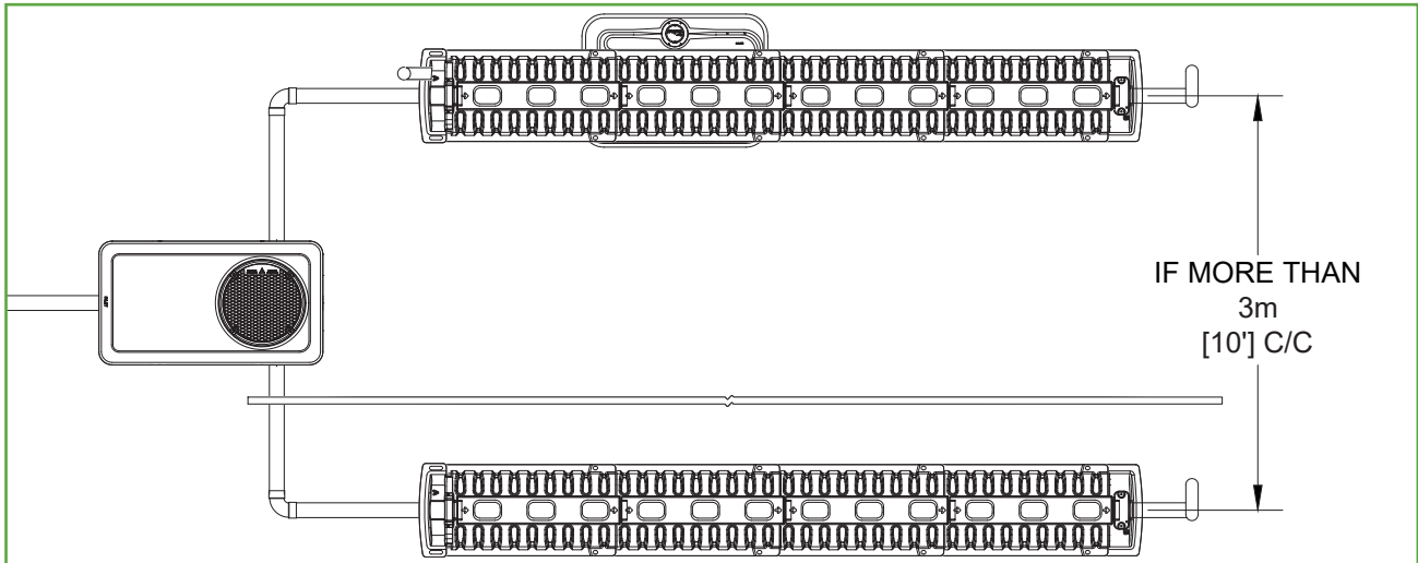
Figure 3: Configuration recommended for system with >3m (10') between runs – Vent between each run
