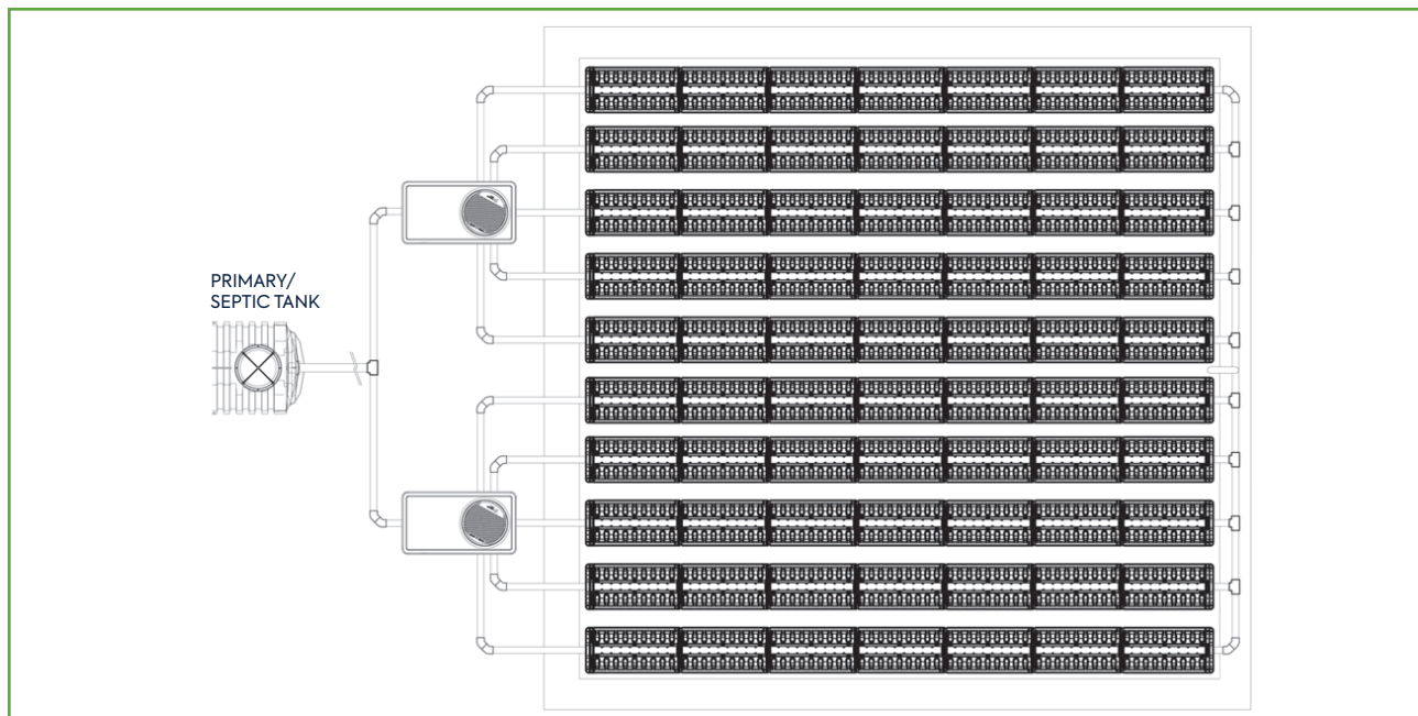
Figure 3.5.1.1 | Ten treatment lines installation fed by two dosing devices
