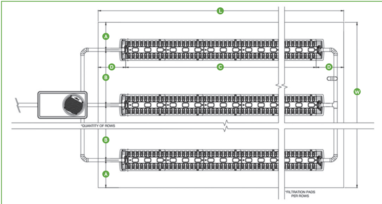
Figure 5.3.1.1 | Typical bed layout — Slope between 0 to 4%
