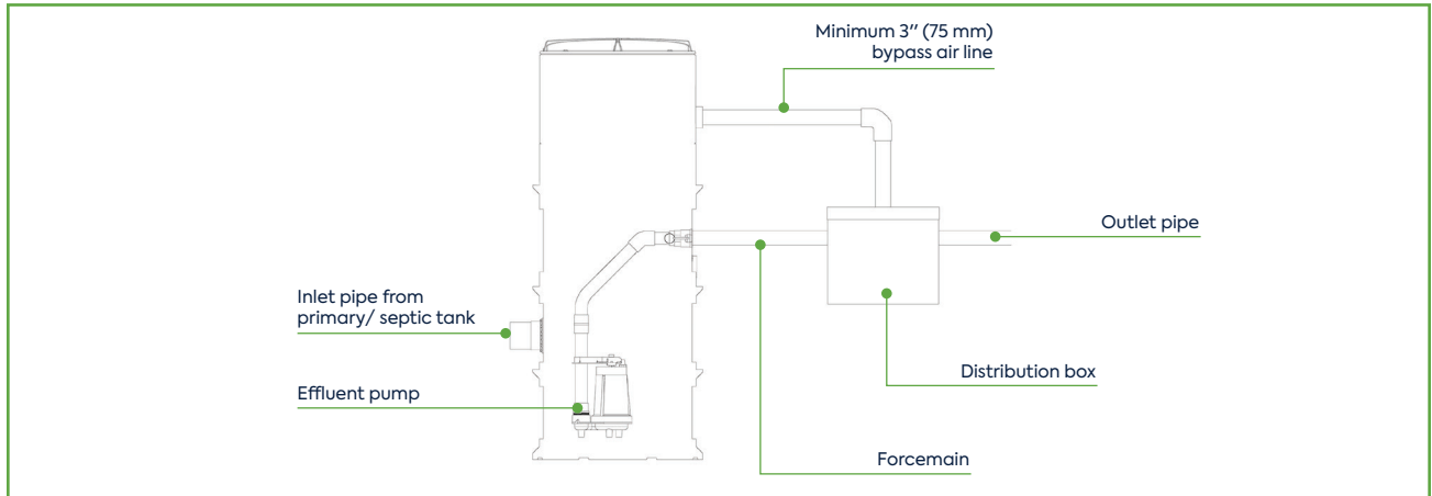
Figure 5.4.1 | Pump-to-gravity installation schematic
